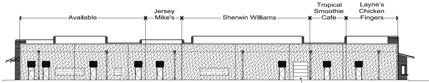
4 NORTH ELEVATION
