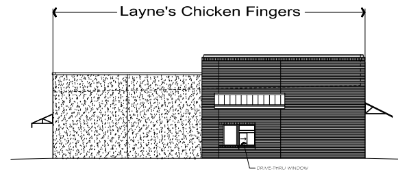
3 WEST ELEVATION
