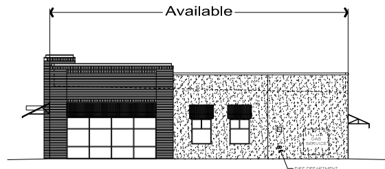
2 EAST ELEVATION
